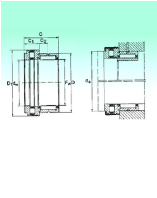
NKXR 35 Bearing 2D drawings and 3D CAD models
